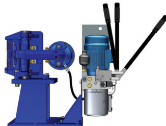
Standard GMRSH Disc Brake Caliper Package
