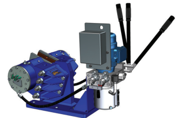
Standard VKSD Disc Brake Caliper Package
